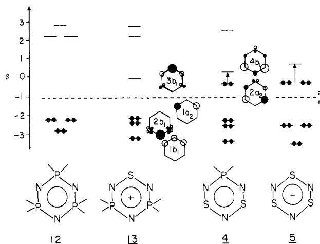
Figure 3. Hückel MO energy levels for the heterocyclic series P x S x-3 N 3 (x = 0-3); α P = +2, α S = -1, α N = -2, β = -1) showing the frontier orbitals for PS 2 N 3 (4) and the three occupied orbitals and the LUMO for P 2 SN 3 + (13). The dotted line separates π and π* orbitals.
