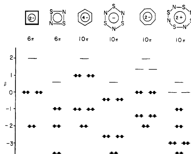
Figure 2. Hückel MO energy levels for S 2 N 2 , S 3 N 3 - , S 4 N 4 2+ , and their hydrocarbon analogues. The carbon p atomic orbital, α C , is arbitrarily chosen as zero energy and α S = -1, α N = -2, β = -1.
